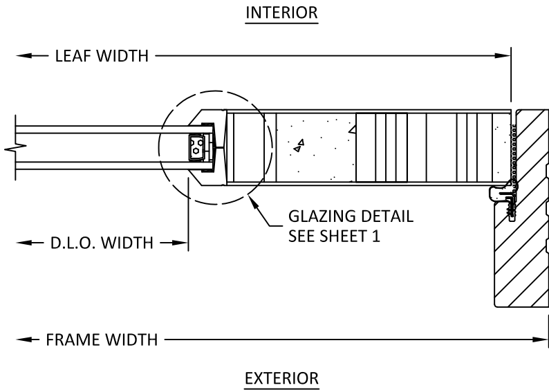
E 4 HORIZONTAL SECTION DOOR LOCK JAMB
