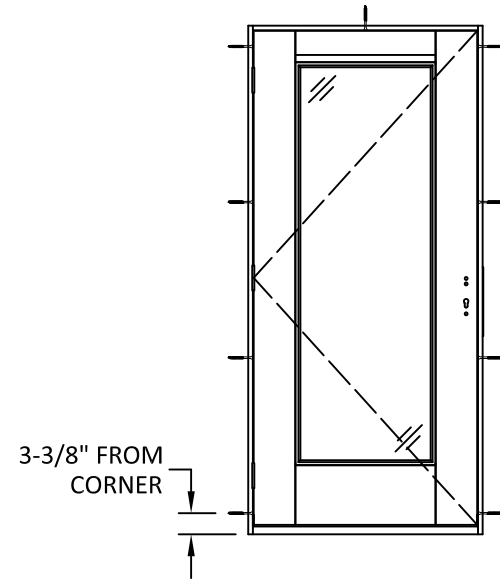
ANCHOR LAYOUT
