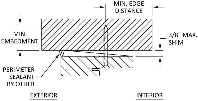
F 5 INSTALLATION DETAIL DOOR HEAD HEAD SHOWN, JAMB SIMILAR
