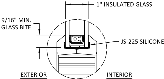
GLAZING DETAIL
