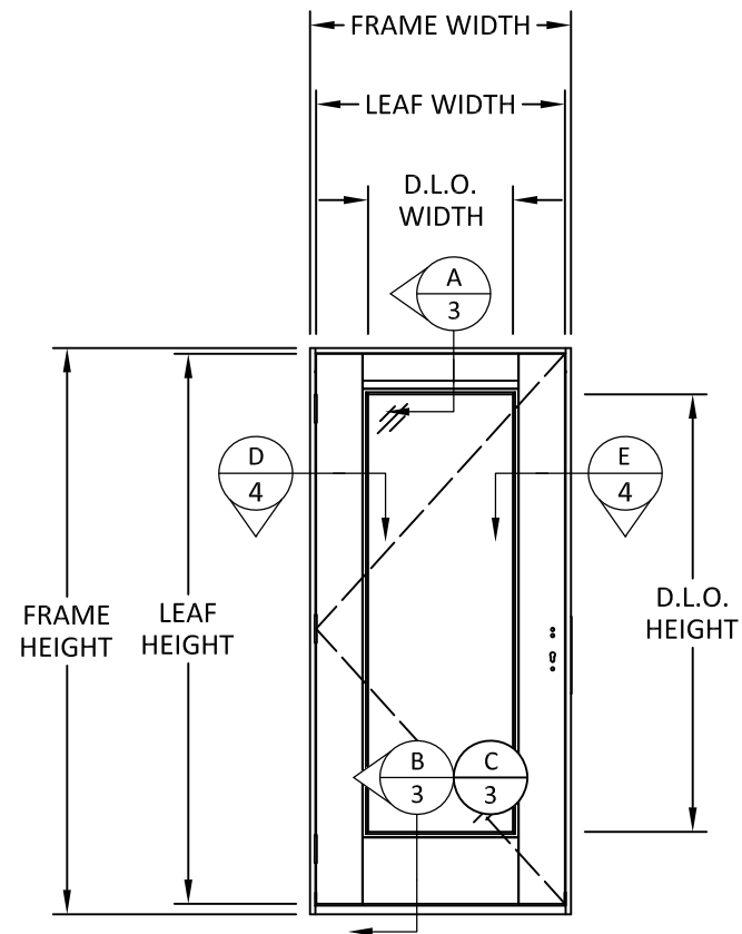
TYPICAL ELEVATION
